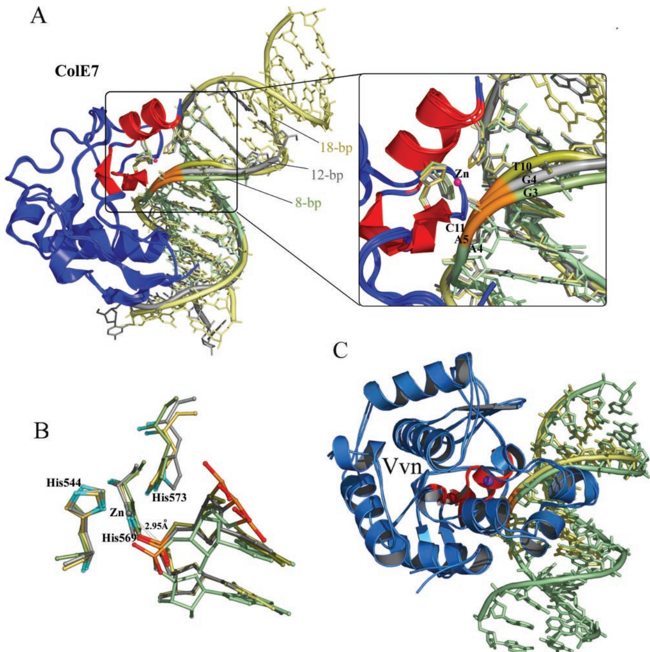
Figure 5. Superposition of three N-CoIE7–DNA complexes and two Vvn–DNA complexes. (A) The crystal structures of the three N-CoIE7–DNA complexes, the preferred complex (18 bp: 2IVH) and the non-preferred complexes (8 bp: 1PT3 and 12 bp: 1ZNS), were superimposed by least-square-fitting of the C \alpha -atoms of N-CoIE7 molecules. The three duplex DNA were aligned after fitting with the metal finger motif (displayed in red) bound at the minor groove, inducing DNA to bend slightly away from the enzyme. The DNA backbones are displayed in yellow for the 18 bp DNA, gray for 12 bp DNA and green for 8 bp DNA, but the backbone ribbons of the scissile phosphates are all displayed in orange. A detailed view of the phosphate backbones is shown in the right panel. The DNA backbone is distorted the most in the preferred complex with a thymine base (T10) located at the 3'-O side of the scissile phosphate as compared to the backbones in the non-preferred complexes, which contain a guanine base before the scissile phosphates (G4 in the 12 bp complex and G3 in the 8 bp complex). (B) Superposition of the active sites in the three N-CoIE7–DNA complexes shows that the scissile phosphate is located closer to the endonuclease active site in the preferred complex (18 bp) with a distance of 2.95 Å between the zinc ion and phosphorus atom. (C) The crystal structures of Vvn–DNA complexes, 8 bp (PDB: 1OUP) and 16 bp (this study, PDB: 2IVK) complexes, were superimposed by a least-square-fit of the C \alpha atoms in Vvn. The DNA backbones fitted well and were not distorted, consistent with Vvn's low sequence-dependent endonuclease activity. Vvn are displayed in blue with metal finger motifs in red. The 16 bp DNA is displayed in green and 8 bp DNA is displayed in yellow.
