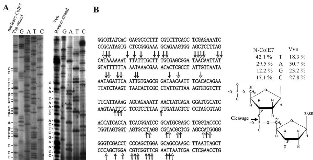
Figure 1. Sequence-dependent DNA cleavage by ColeE7 and Vvn. (A) The 5'- 32 P-labeled PCR-amplified 260 bp DNA fragments (0.7 μM) were incubated respectively with 4 μM Zn 2+ -bound N-ColeE7 and 30 nM Vvn in the presence of 2 mM Mg 2+ and 20 mM Tris-HCl buffer (pH 8) at 37°C for 5 min. The reaction was terminated by adding 10 mM EDTA. The cleaved products were separated by gel electrophoresis in 8% denaturing polyacrylamide gel with the sequencing reactions carried out alongside. Only one representative DNA digestion patterns by N-ColeE7 (top strand) and Vvn (bottom strand) are shown here. (B) The sequences of top strand and bottom strand DNA used for footprint assays are listed. The DNA cleavage sites by N-ColeE7 are indicated by arrows. The solid arrows show the cleavage of the 3'O-P bond with a thymidine at the 3'O-side of the scissile phosphate. A schematic diagram shows DNA cleavage by N-ColeE7 with the preference for the base at the 3'O-side of the scissile phosphate: T (41.2%) > A (29.5%) > C (17.1%) > G (12.2%). Vvn is less specific in DNA cleavage with an order of A (30.7%) > G (23.2%) > C (27.8%) > T (18.3%). The cleavage percentage was estimated by first integrating each cleavage band in the autoradiography and normalized by calculating the summation of I_{\text{base}}/N_{\text{base}} divided by the summation of I_{\text{all}} , in which I_{\text{base}} is the band intensity cleaved at a specific base (A, T, C or G), I_{\text{all}} is the band intensity cleaved at all bases and N_{\text{base}} is the number of a specific base in the DNA.
