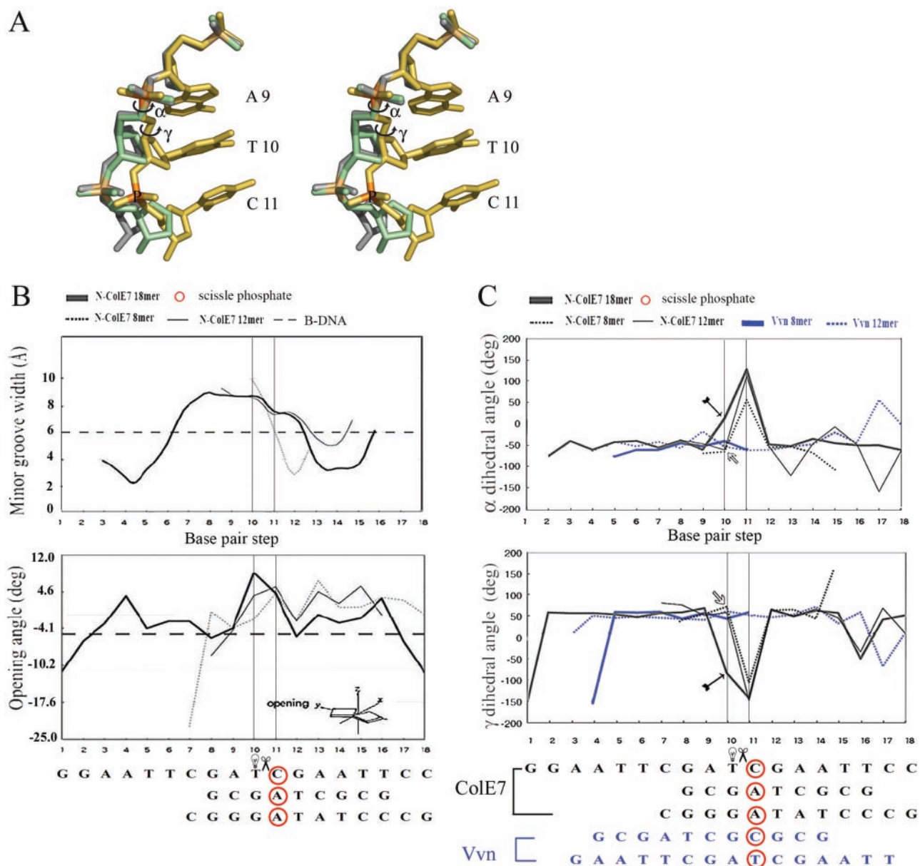
Figure 6. The transitions in \alpha and \gamma dihedral angles before and after the cleavage site result in a larger DNA backbone conformational change in the preferred complex of N-CoIE7–DNA (18 bp) upon enzyme binding to DNA. (A) Stereo view of the superimposed DNA in the three N-CoIE7–DNA complexes shows that a larger phosphate backbone conformational change observed only in the preferred complex is resulted from the transitions in \alpha and \gamma dihedral angles upon the enzyme binding to the preferred DNA site. The phosphate backbones are shown in green for the 8 bp DNA, gray for the 12 bp DNA and yellow for the 18 bp DNA; only the bases of A9, T10 and C11 in the 18 bp DNA are shown. The transitions in \alpha and \gamma dihedral angles before the cleavage site in the preferred 18 bp complex are marked by circled arrows. (B) The minor groove widths in the three complexes (8 bp: IPT3, 12 bp: IZNS and 18 bp: 2IVH) are all widened to \sim 9 Å as compared to a canonical B-form DNA. The base pair opening angles are slightly higher in the widened minor groove regions in the preferred complex (18 bp) than those of the non-preferred complexes (8 and 12 bp). (C) The \alpha and \gamma dihedral angles immediately before and after the cleavage site have non-canonical values only in the preferred 18 bp complex (marked by arrows in the figure). The \alpha/\gamma before the cleavage site are 39.4^\circ/-89.4^\circ for 18 bp complex, -61.9/59.1^\circ for 12 bp complex and -56.6/46.0^\circ for 8 bp complex. The transitions in \alpha and \gamma upon protein binding to the preferred site lead to the DNA backbone conformational change observed in the preferred complex.
