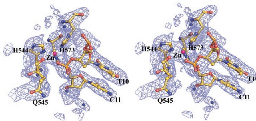
Figure 2. Stereo view of the electron density map of N-ColeE7-DNA (18 bp) complex at active site. The omit map ( F_o - F_c ) contoured at 2.5 \sigma was calculated after omitting the active site atoms in the refinement model. The electron density of the mutated residue H545→Q and zinc ion can be clearly visualized. The scissile phosphate between T10 and C11 is coordinated to the zinc ion.
